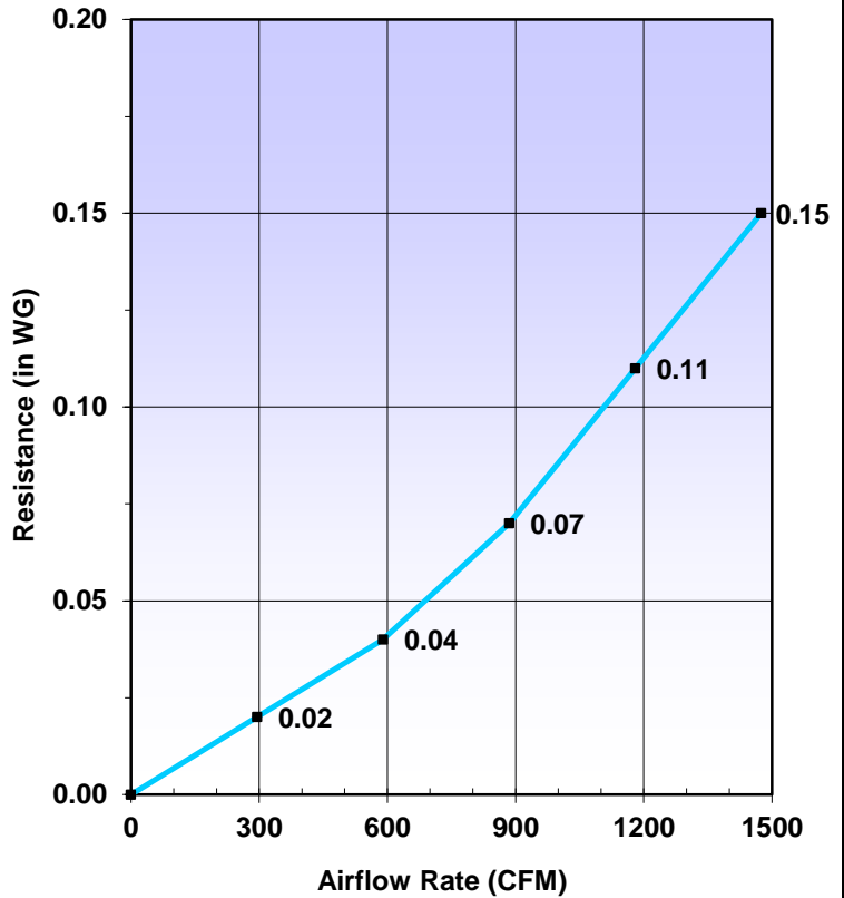
Air Flow vs Resistance
